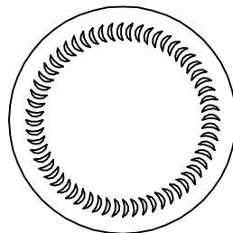
VIEW ON BASE STANDING AREA EMBOSED WITH TURBINE STIPPLE.
